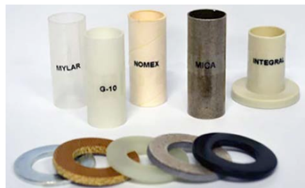
Isolating Sleeves & Washers
